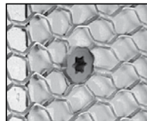
Wire lath to steel or wood studs.
